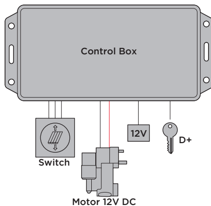
THULE MOTOR 12V TECHNICAL SPECIFICATIONS
